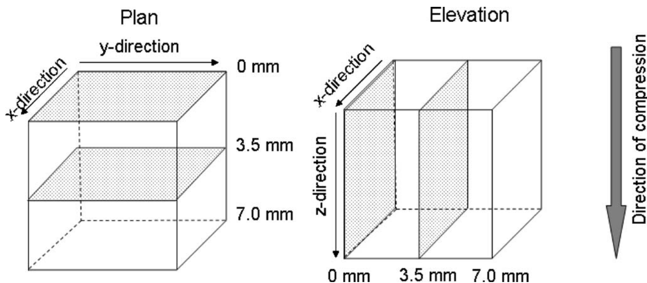
Fig. 1. The locations of the plan images ( left ) and of the elevation images ( right ) in the cubic compact. Per plane nine images were taken in a 3 \times 3 pattern
