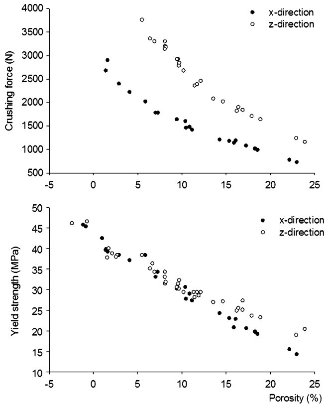
Fig. 3. Crushing force versus porosity (above) and yield strength versus porosity (below), in the x -direction and the z -direction. The porosity was calculated out of weight and volume
