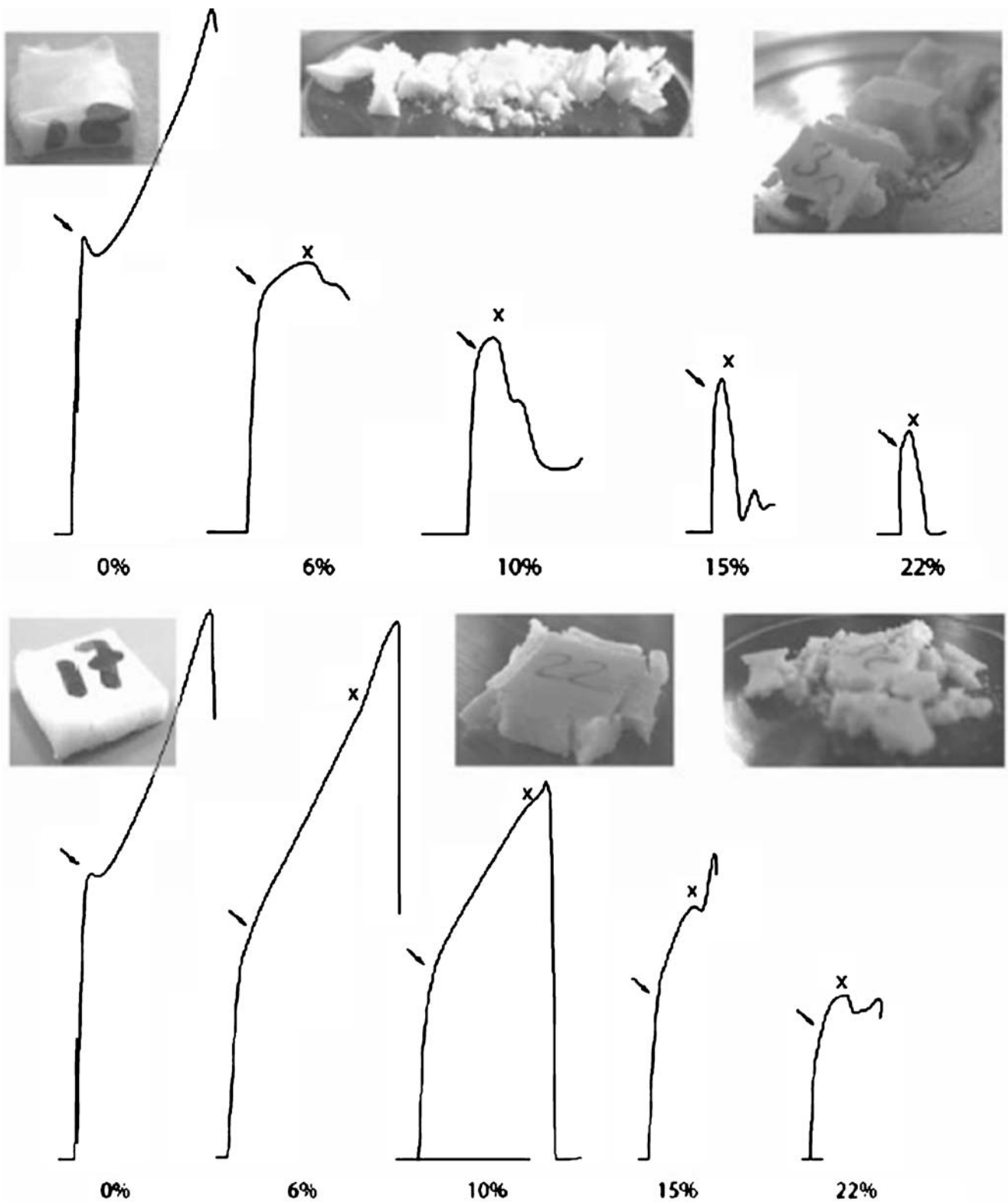
Fig. 2. Force displacement curves of crushing in the x -direction ( above ) and in the z -direction ( below ) of cubes with a different porosity. Arrows indicate yield points and the 'x' indicates where fracture occurred. The images depict cubes after crushing
