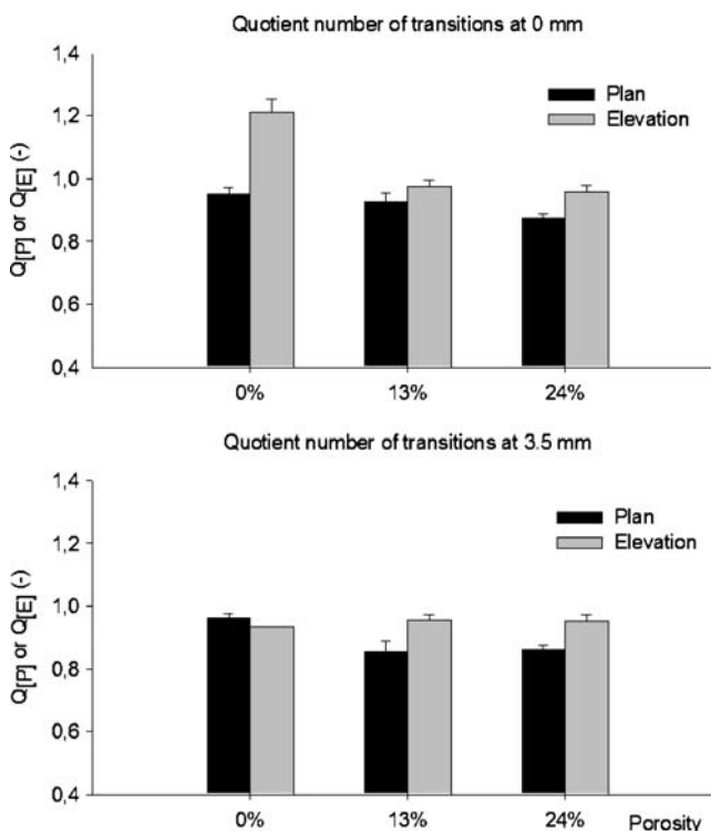
Fig. 6. Quotient of the number of transitions in the plan and elevation images of the compacts of low, intermediate, and high porosity from the plane at 0 mm from the side of the cube ( above ) and from the plane at 3.5 mm from the side ( below )
